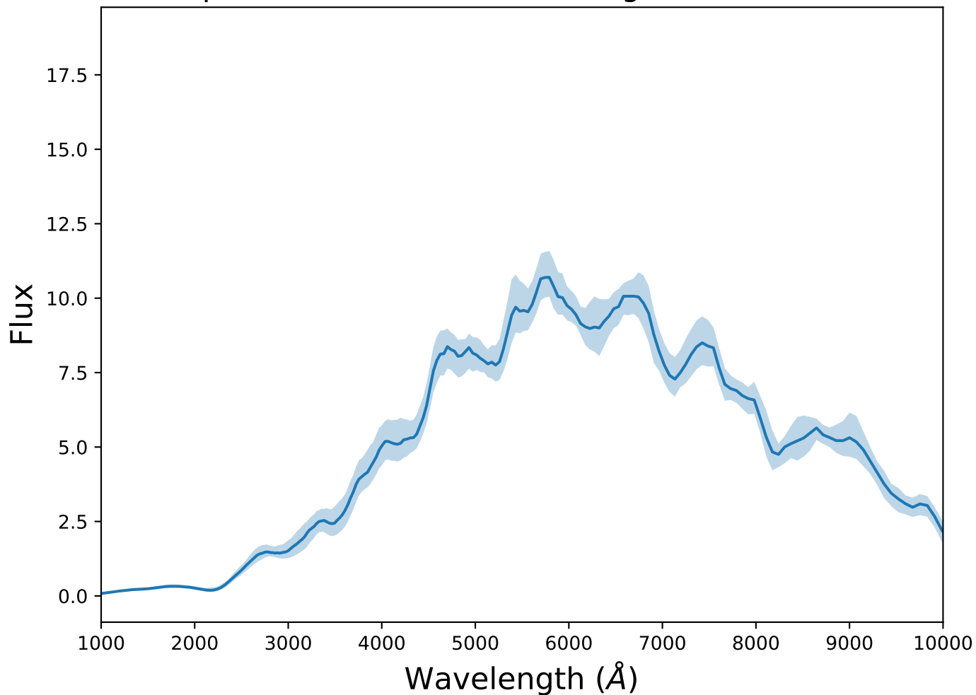
Spectrum 5 for transient 91bg-like at z=0.32
